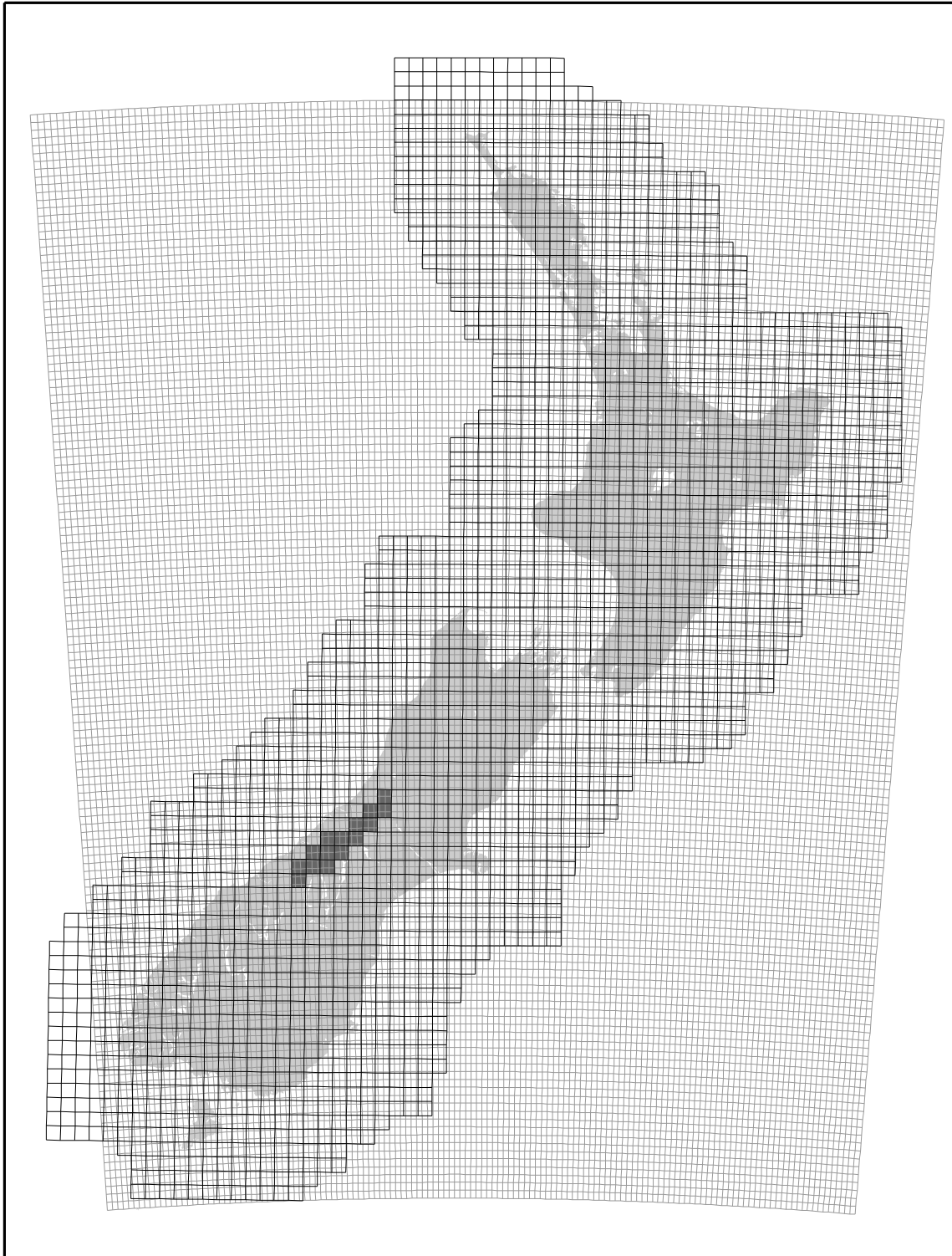
Figure 3: The coarse grid shown is the 20km grid of points on which the distortion model was calculated. The shaded cells are those on which the distortion constraint on the cells was downweighted to account for the difference between the original NZGD49 definition on the east of the South Island and the later extension on the West Coast. The distortion model was interpolated onto the finer grid for publication.
