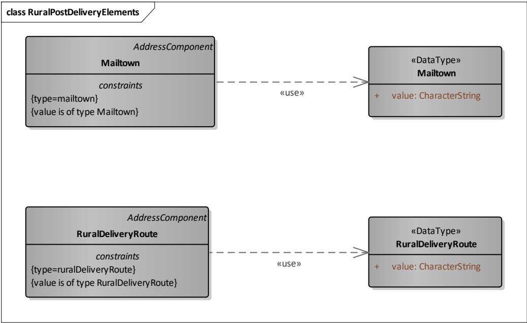
Figure 10: RuralPostDeliveryElements
