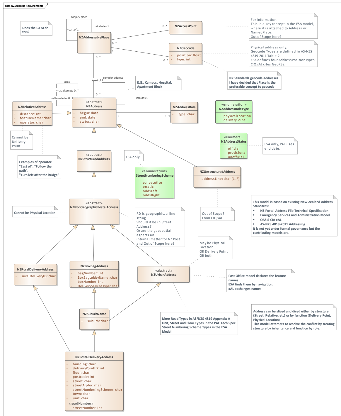
Figure 22: Merged elements of address documents
