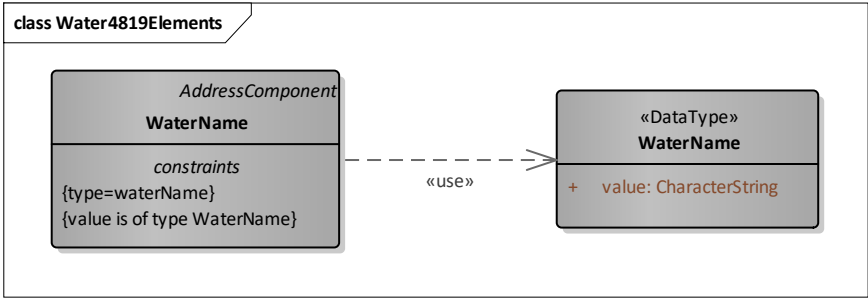
Figure 13: Water4819Elements
