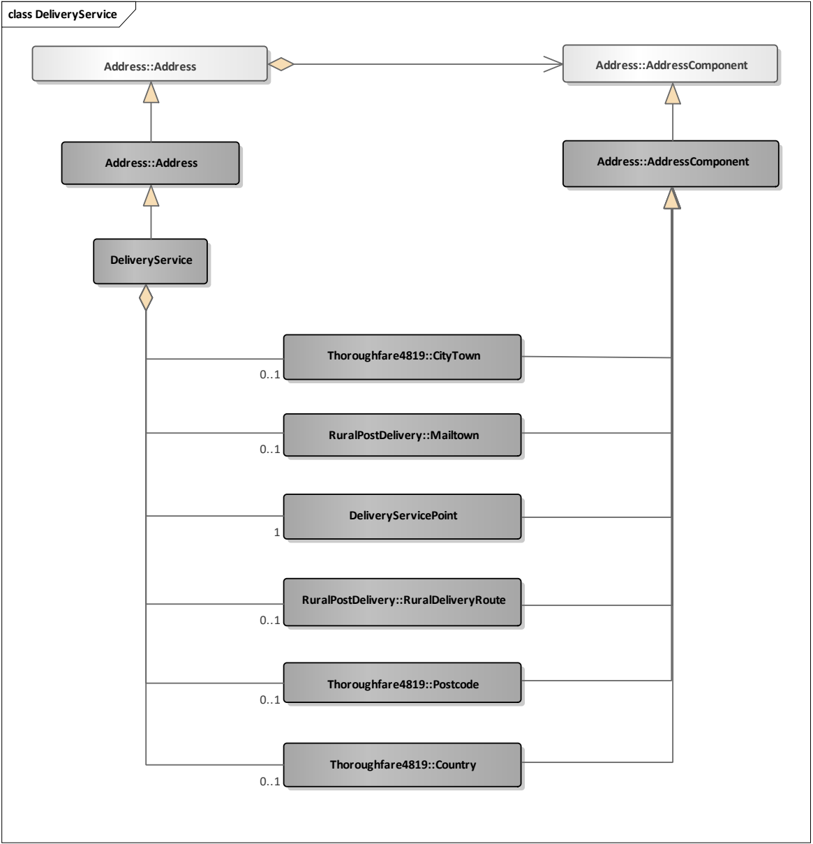
Figure 14: DeliveryService.
