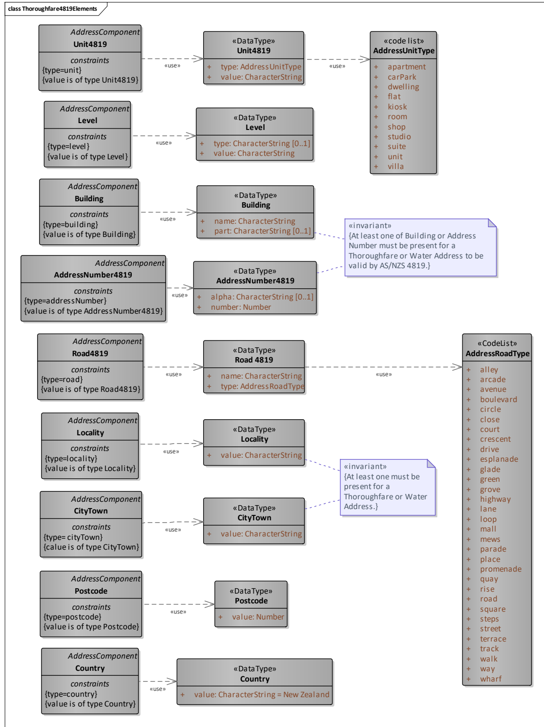
Figure 12: Thoroughfare4819Elements
