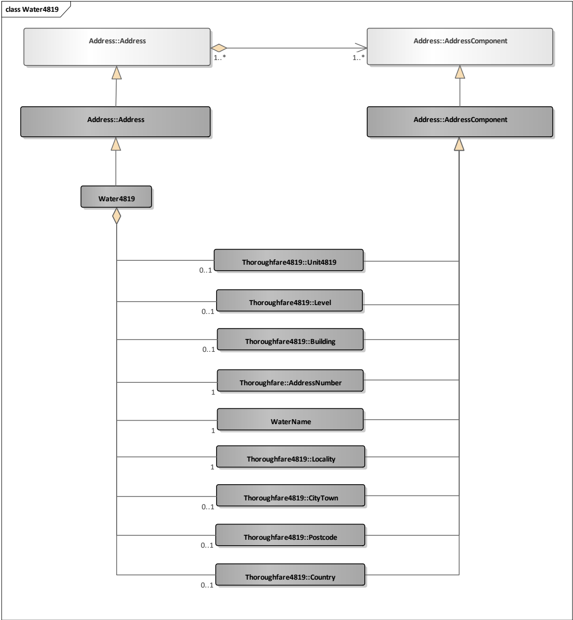
Figure 19: Water4819
