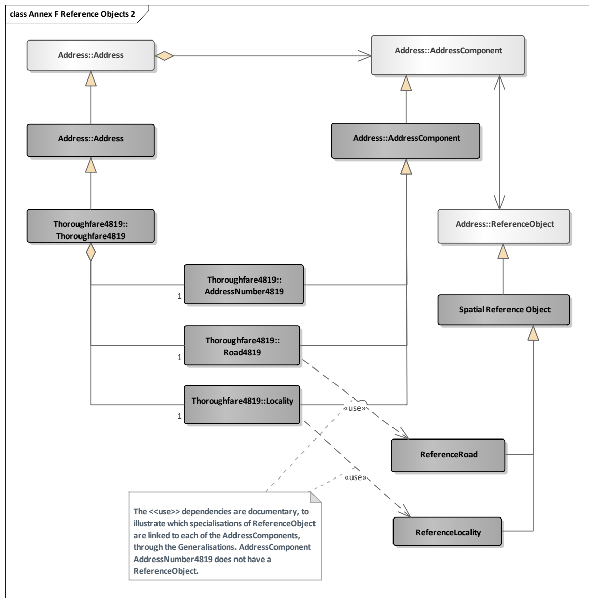
Figure 24: Reference Object applied to Throughfare address class
