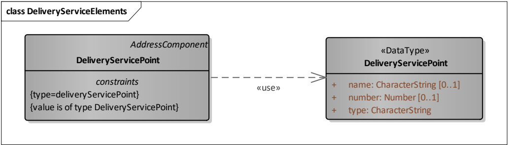
Figure 9: DeliveryService elements
