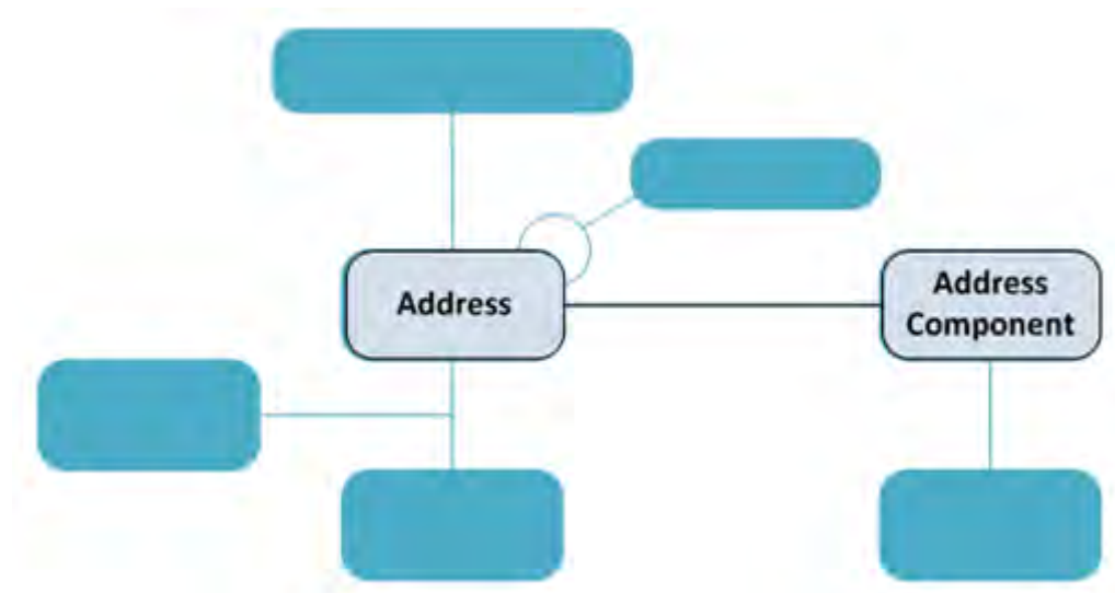
Figure 1: Foundation elements
