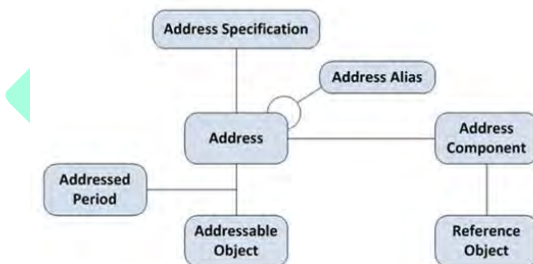
Figure 2: Additional elements
