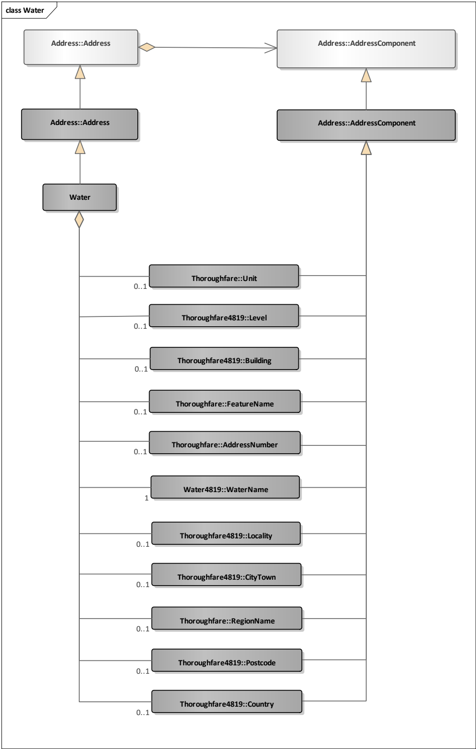
Figure 18: Water
