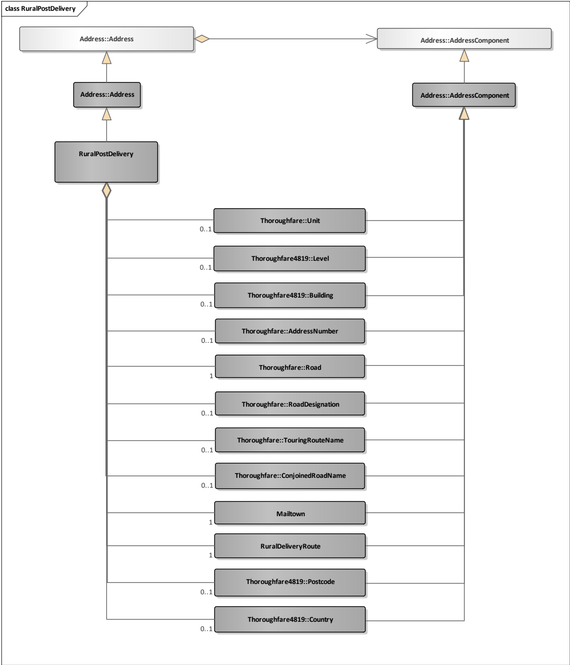
Figure 15: RuralPostDelivery
