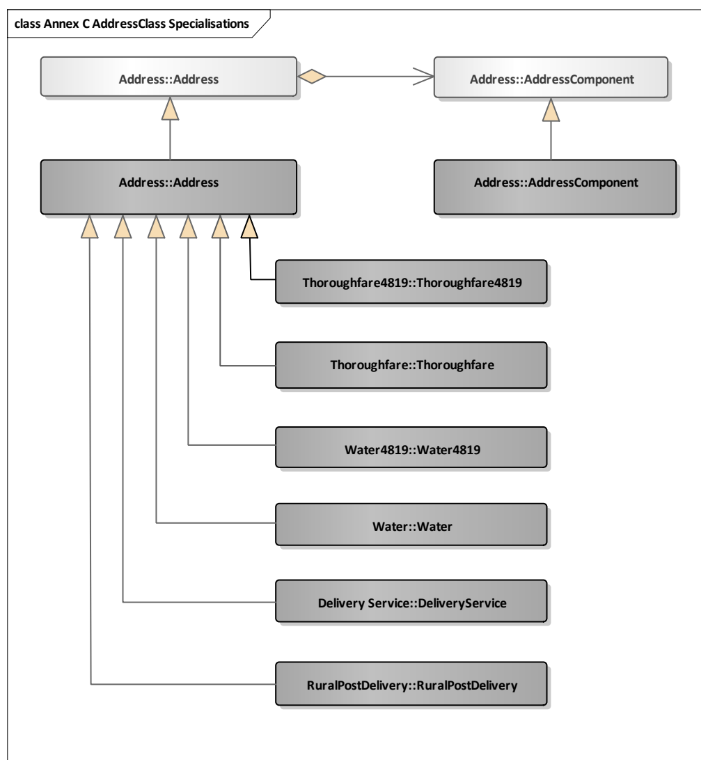
Figure 8: AddressClass specialisations
