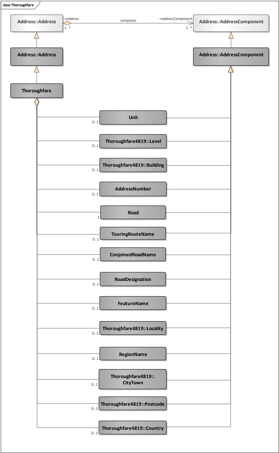
Figure 16: Thoroughfare
