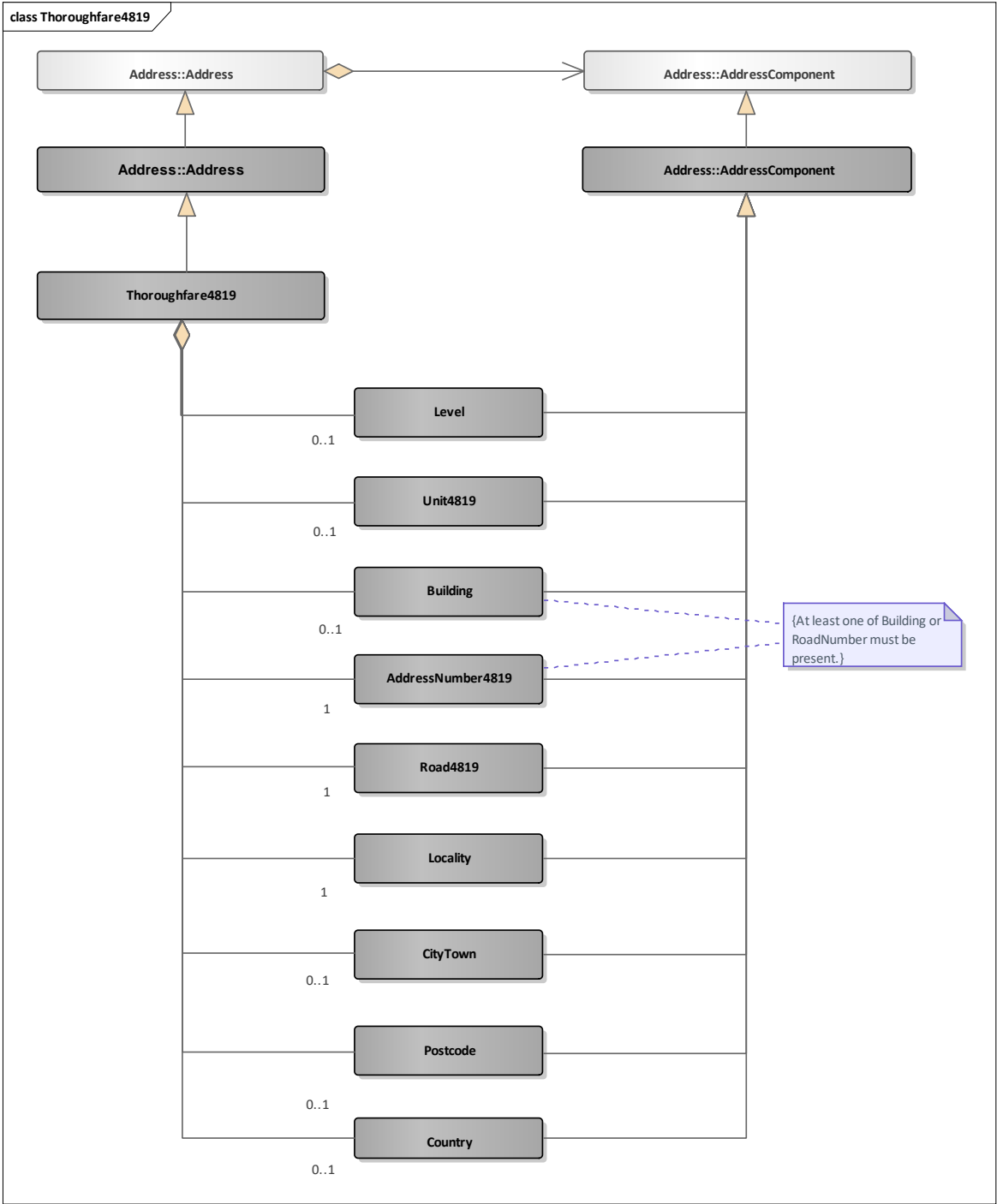
Figure 17: Thoroughfare4819
