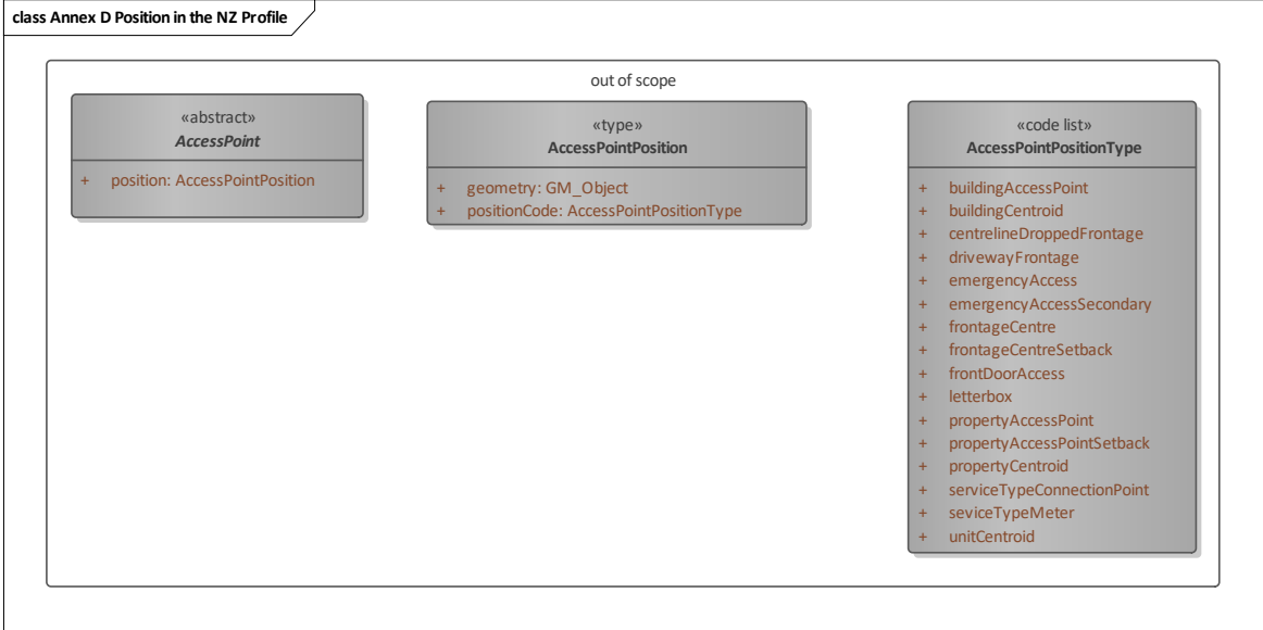
Figure 21: Teatment of position
